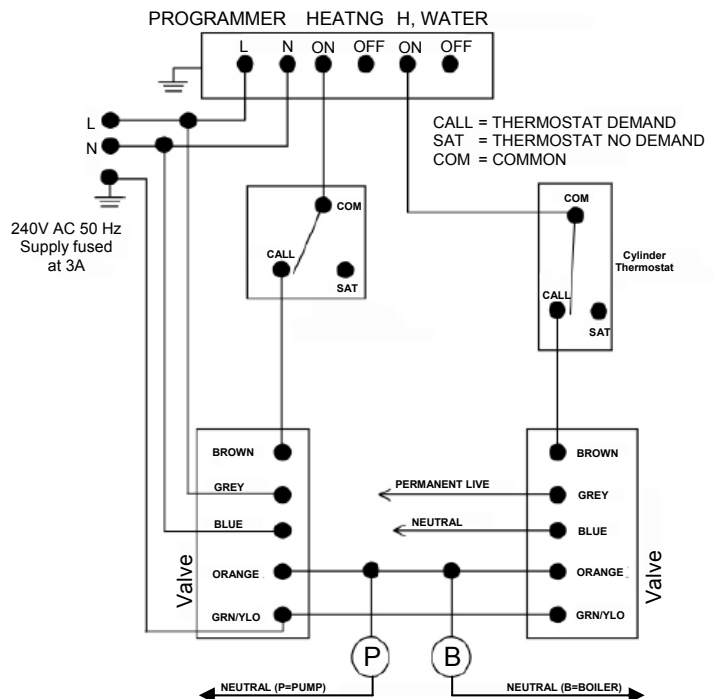
Typical circuit using two zone Valves ZV22 Programmer, Room Thermostat and Cylinder Thermostat
